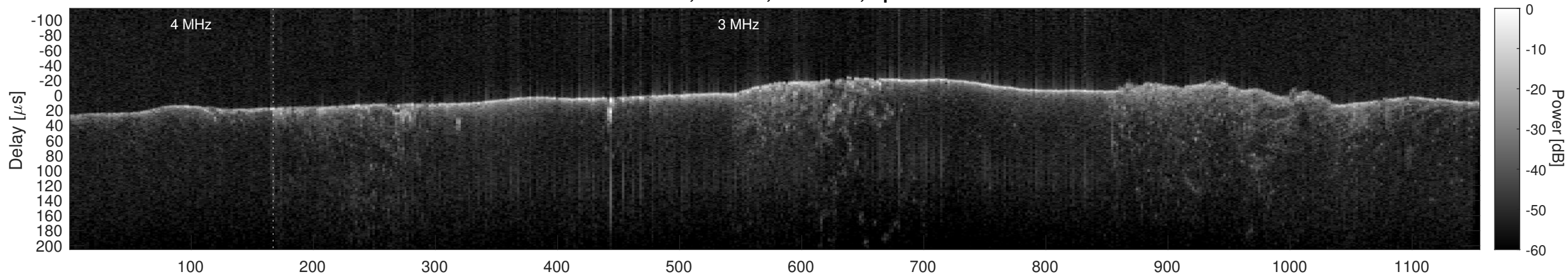
Orbit 15528, Cluttergram
