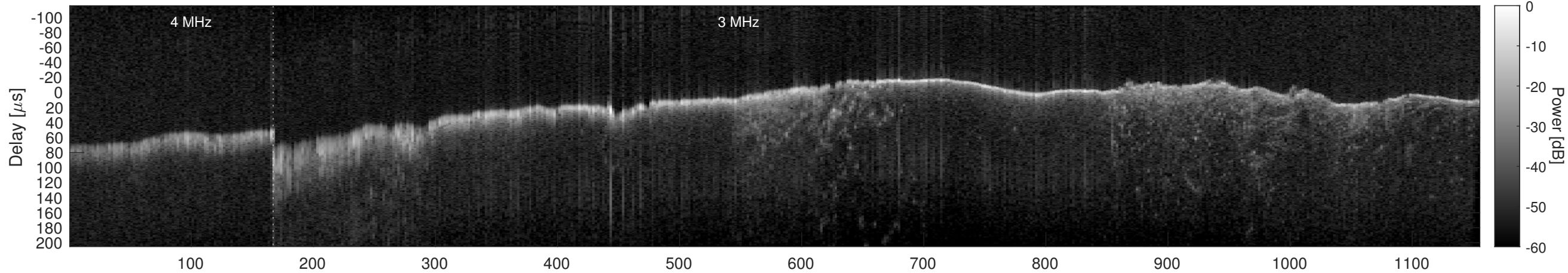
Orbit 15528, Window, Channel 2, Chapman
