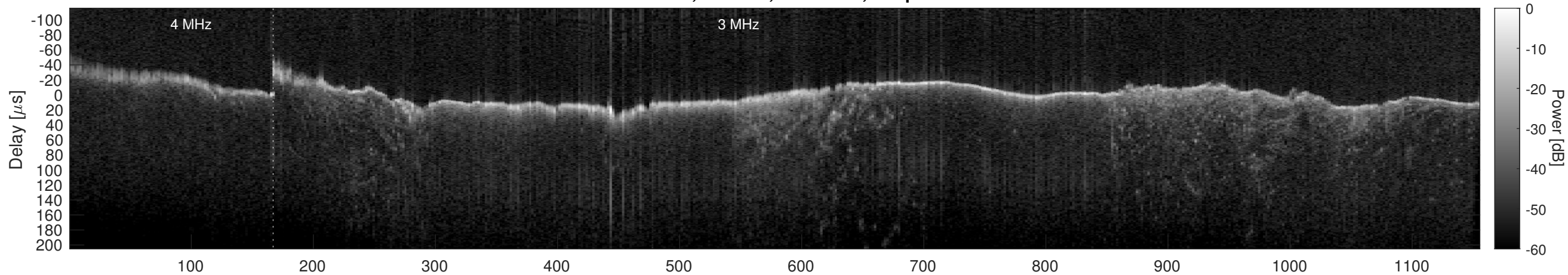
Orbit 15528, Window, Channel 2, Optimized
