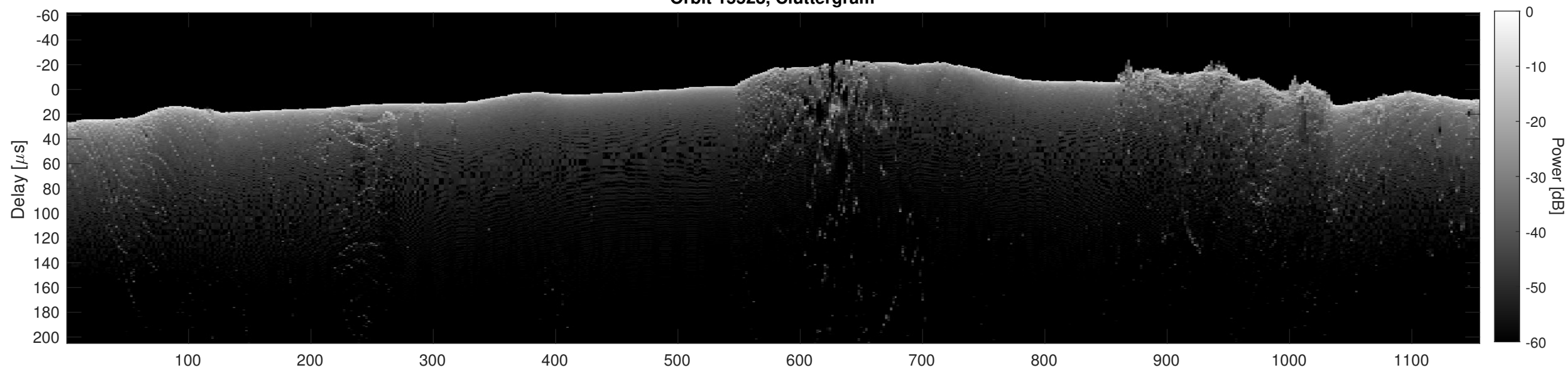
Orbit 15528, Cluttergram
