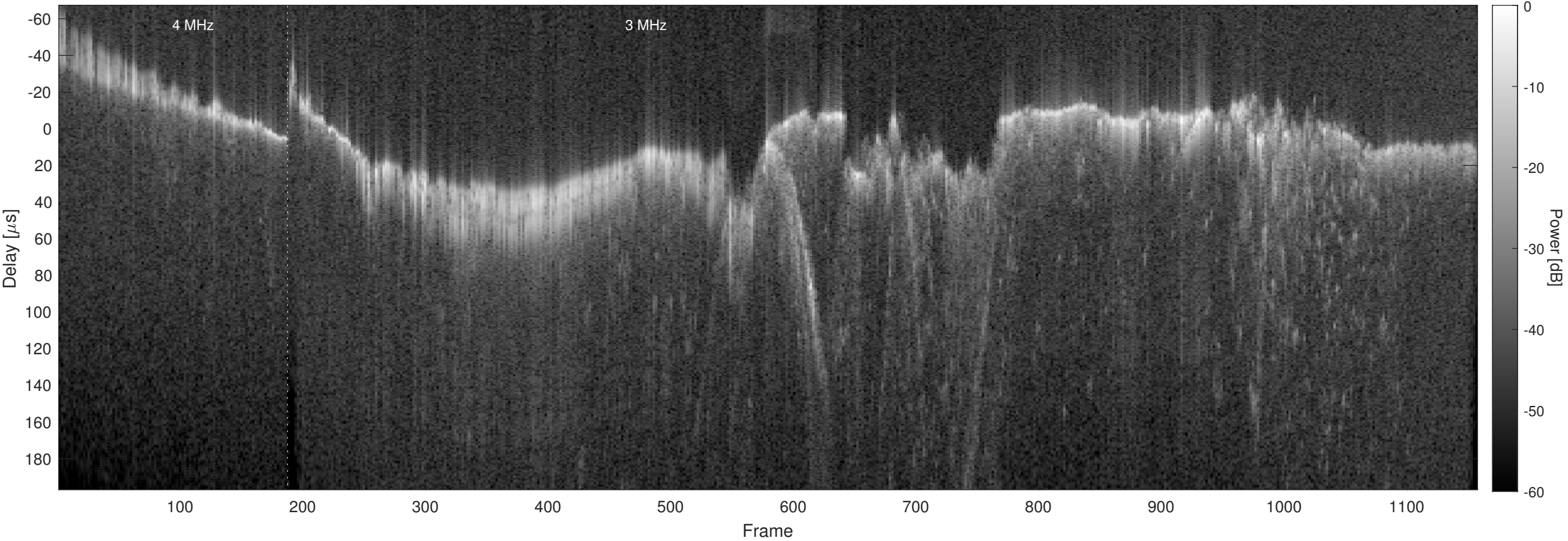
Orbit 15531, Chapman, No Window, Channel 2
