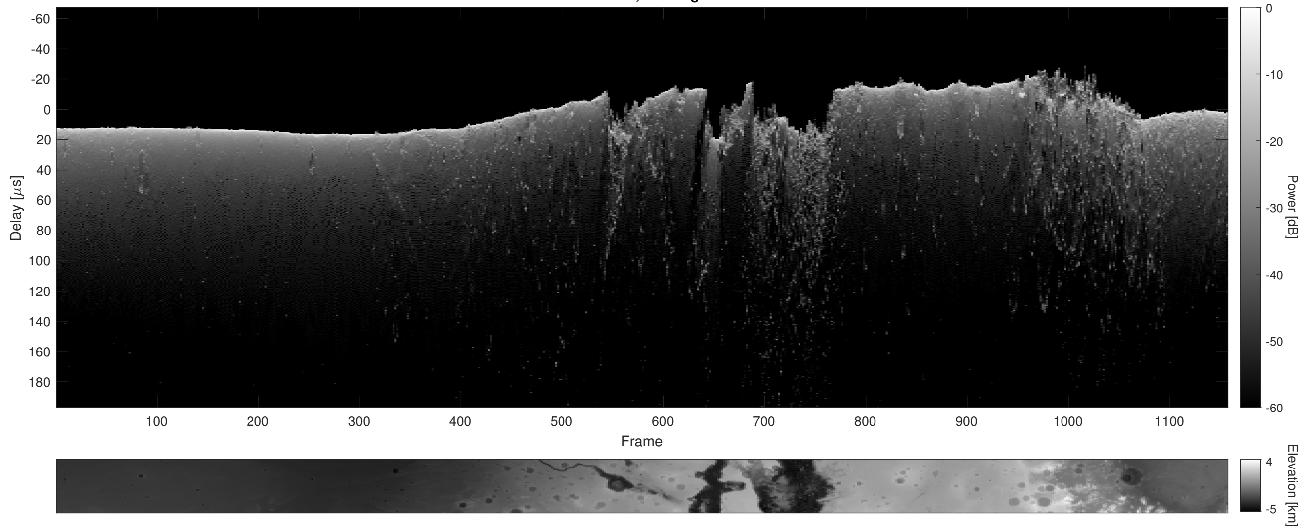
Orbit 15531, Cluttergram
