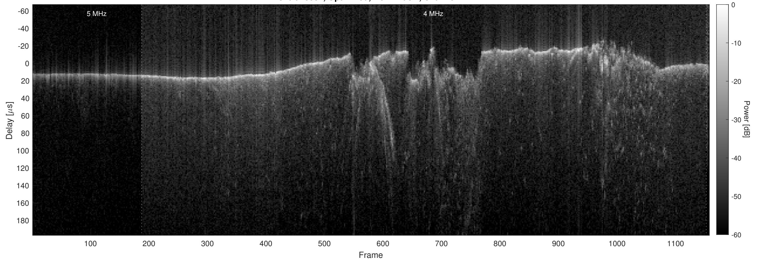
Orbit 15531, Optimized, No Window, Channel 2
