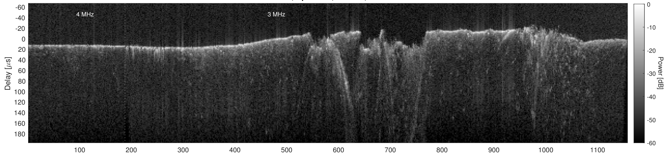
Orbit 15531, Cluttergram
