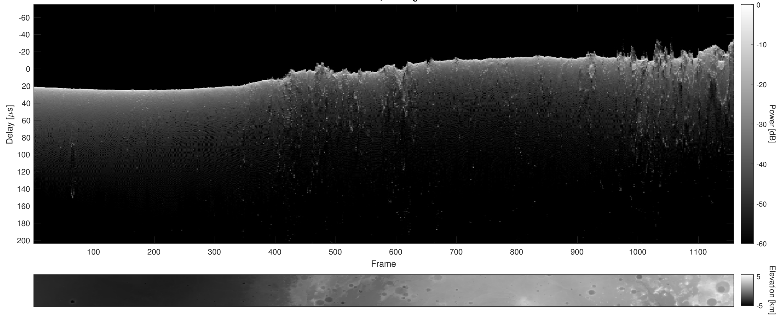
Orbit 15533, Cluttergram
