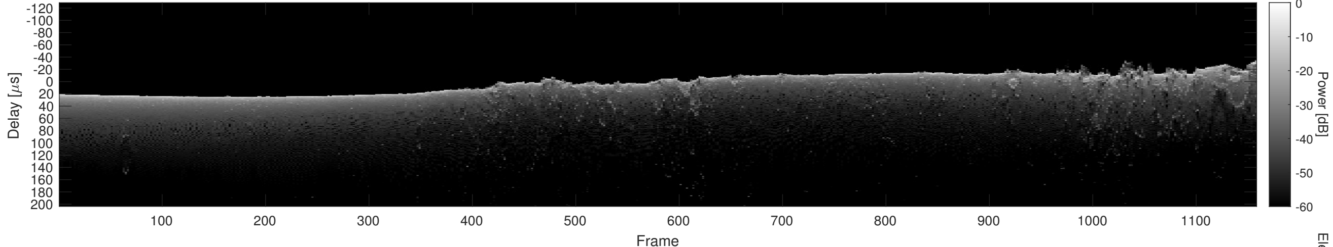
Orbit 15533, Cluttergram
