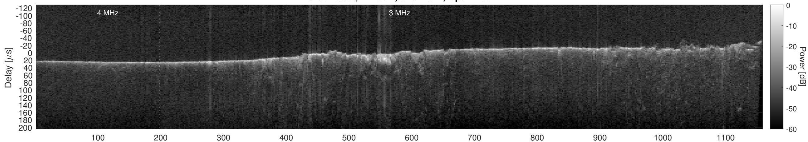
Orbit 15533, Cluttergram
