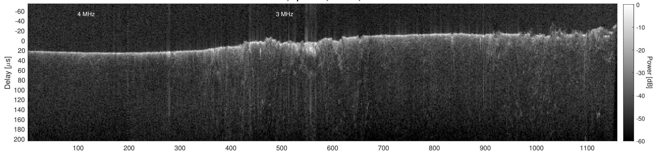
Orbit 15533, Cluttergram
