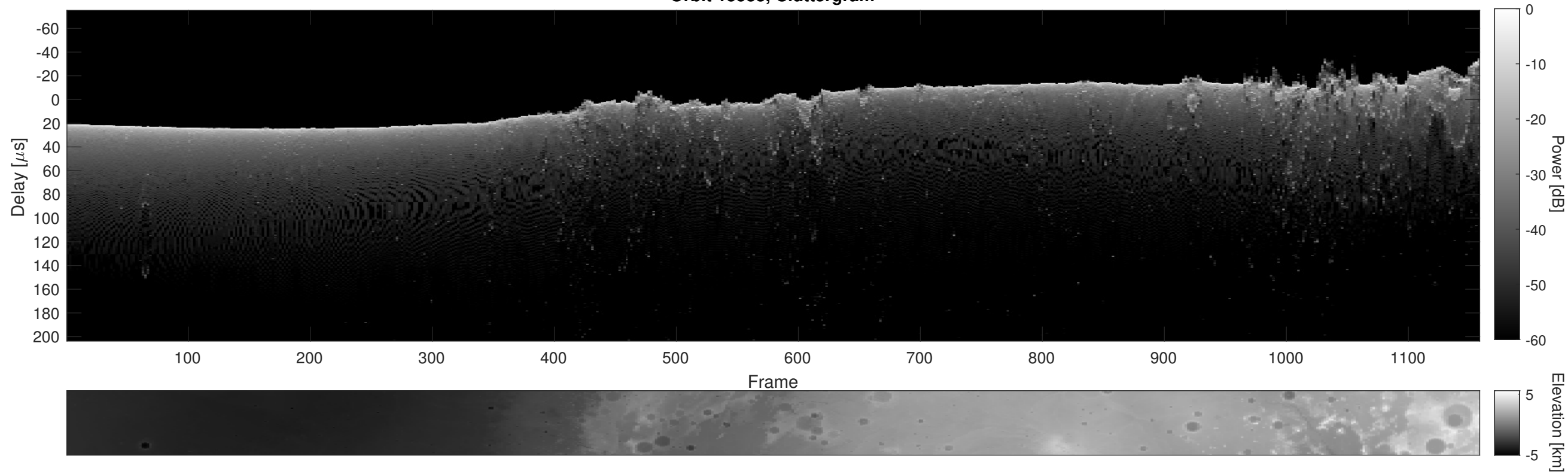
Orbit 15533, Cluttergram
