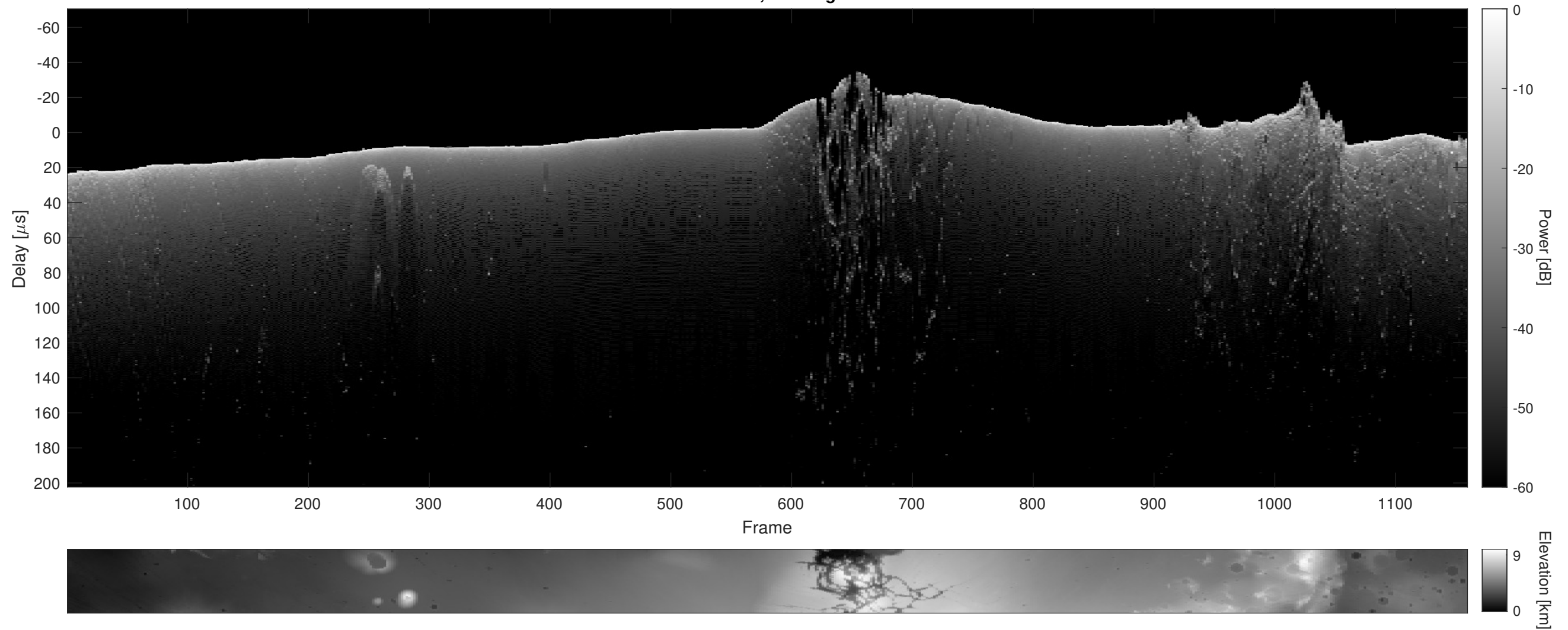
Orbit 15535, Cluttergram
