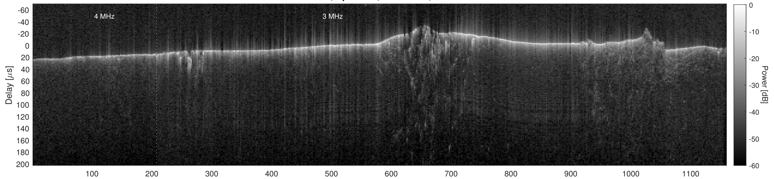
Orbit 15535, Cluttergram
