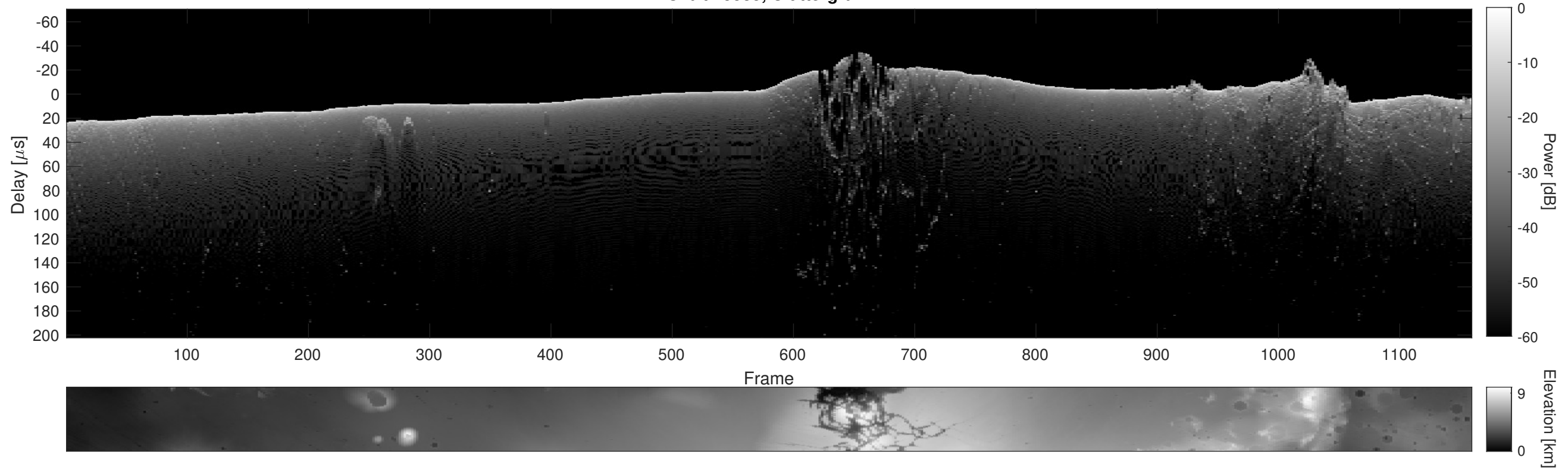
Orbit 15535, Cluttergram
