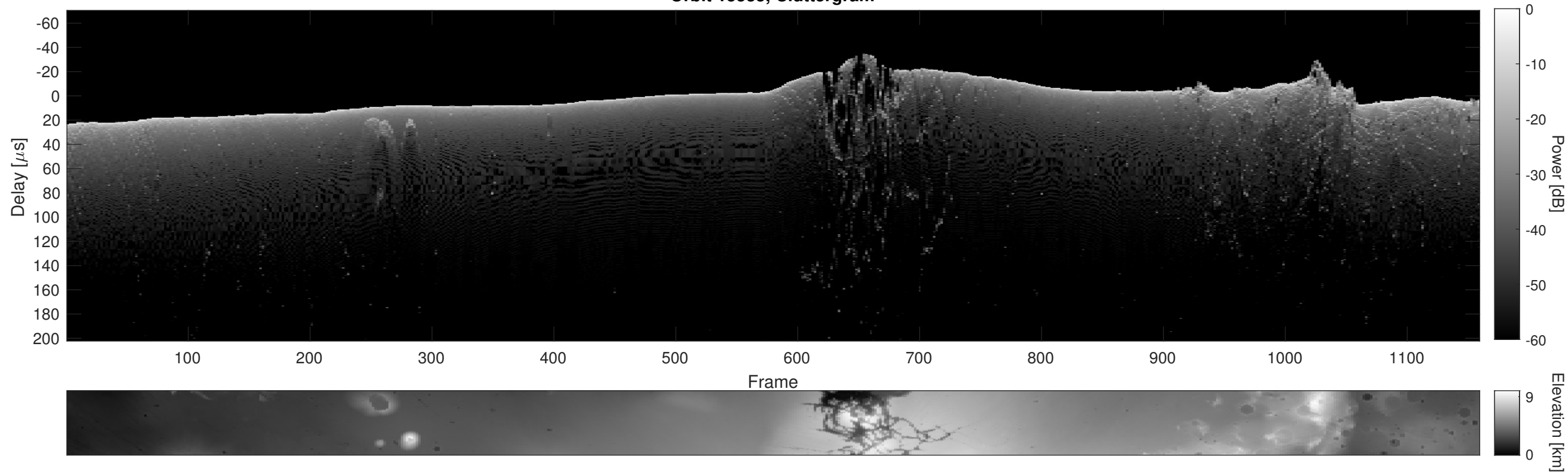
Orbit 15535, Cluttergram
