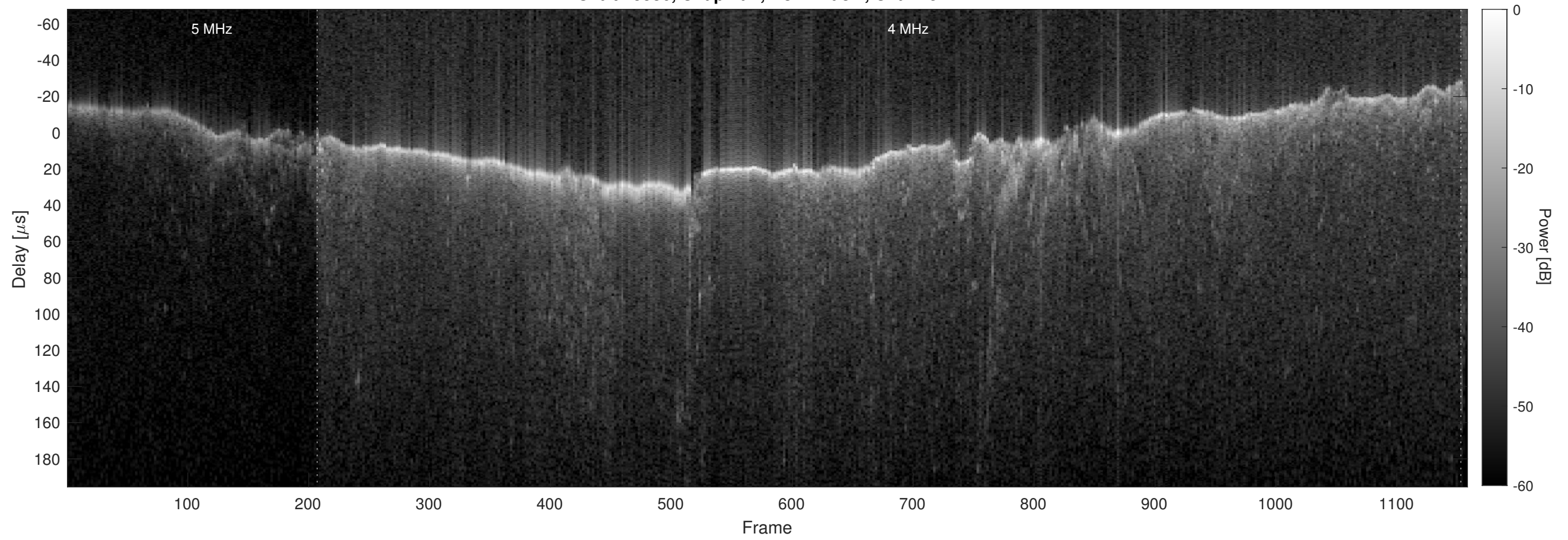
Orbit 15536, Chapman, No Window, Channel 2
