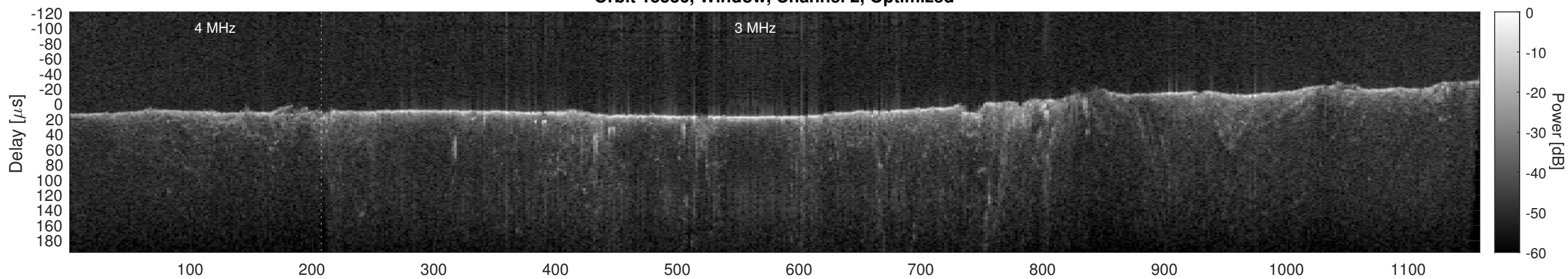
Orbit 15536, Cluttergram
