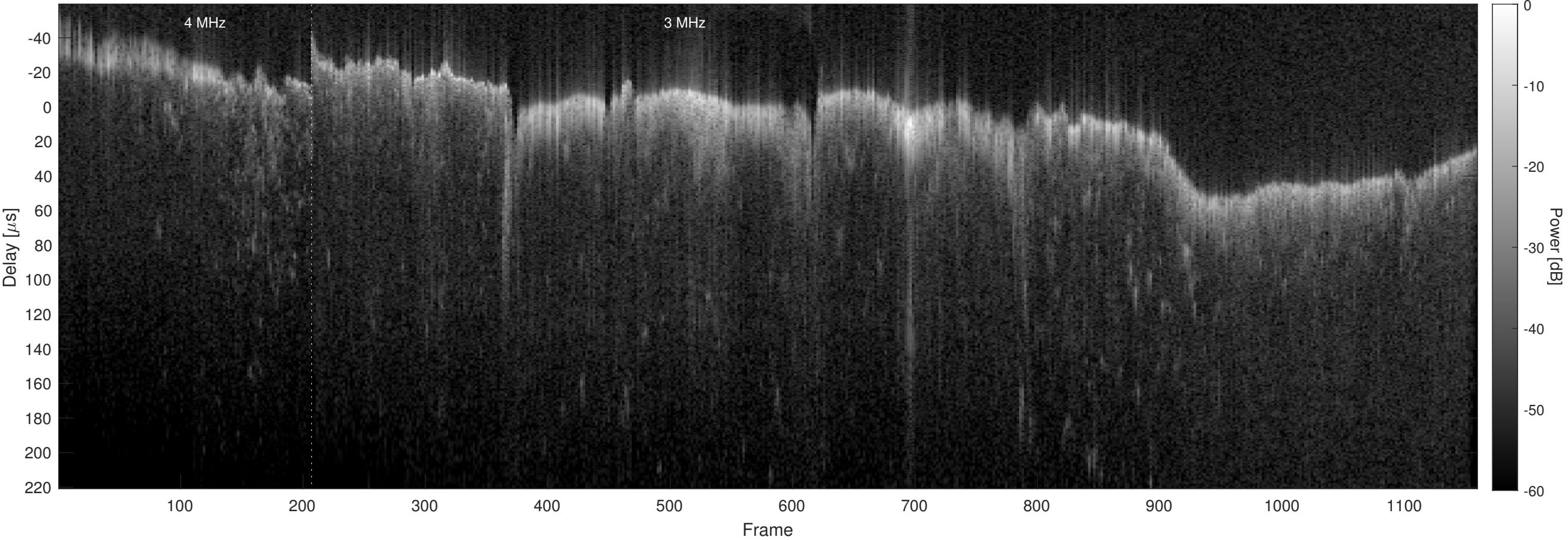
Orbit 15537, Chapman, No Window, Channel 2
