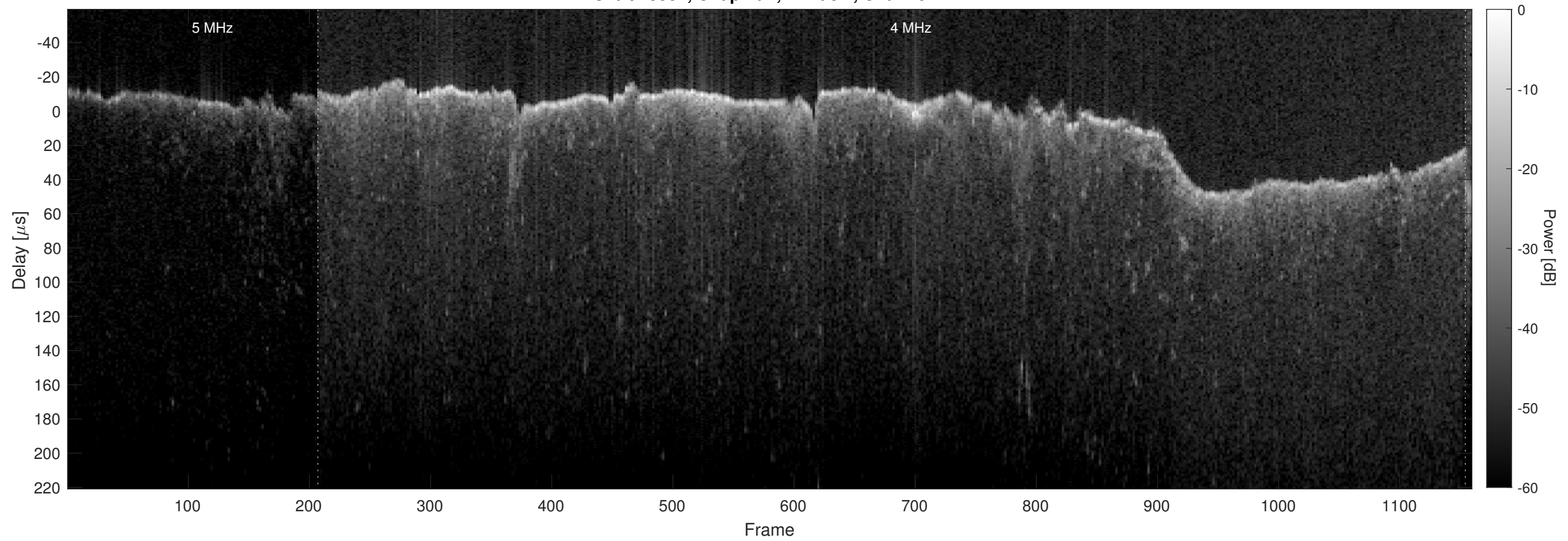
Orbit 15537, Chapman, Window, Channel 2
