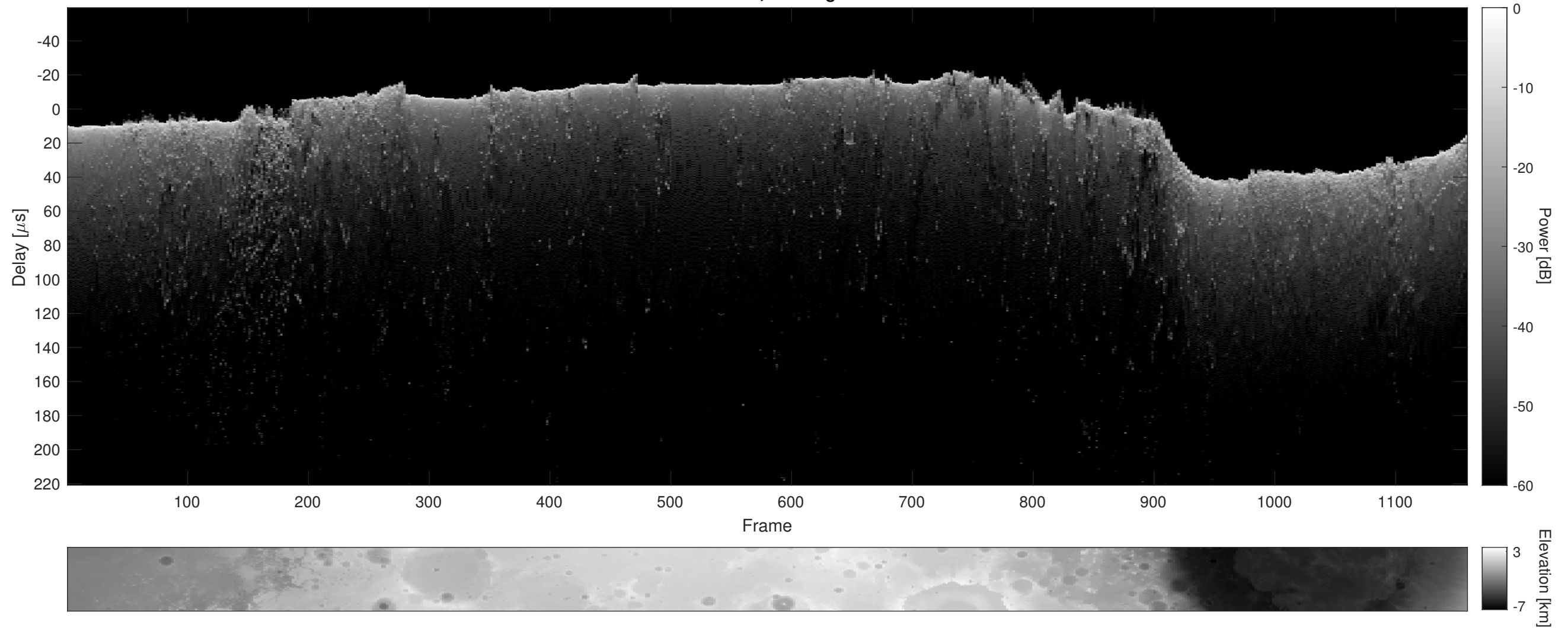
Orbit 15537, Cluttergram
