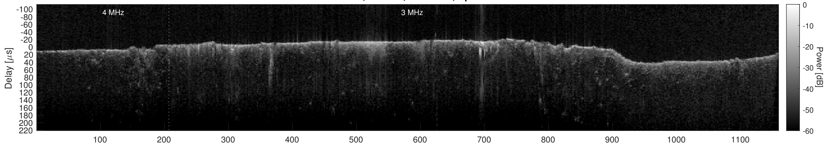
Orbit 15537, Cluttergram
