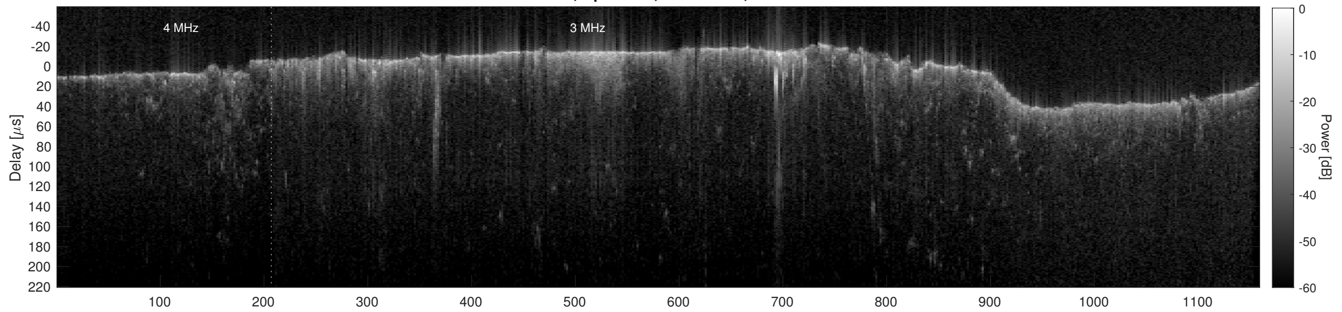
Orbit 15537, Cluttergram
