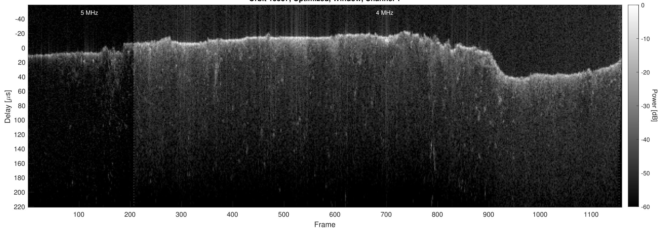
Orbit 15537, Optimized, Window, Channel 2
