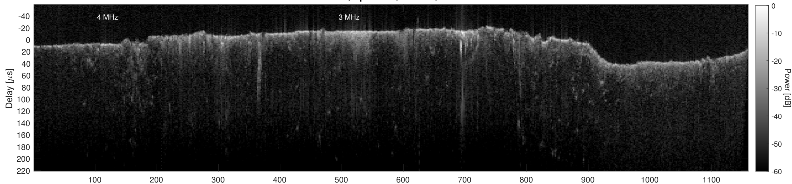
Orbit 15537, Cluttergram
