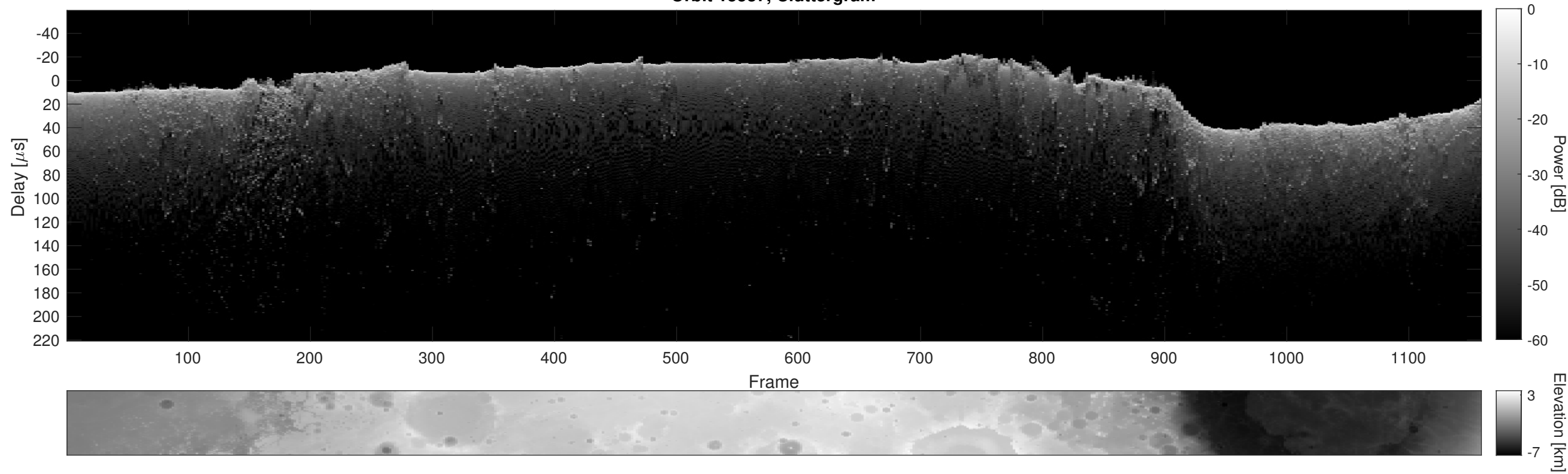
Orbit 15537, Cluttergram
