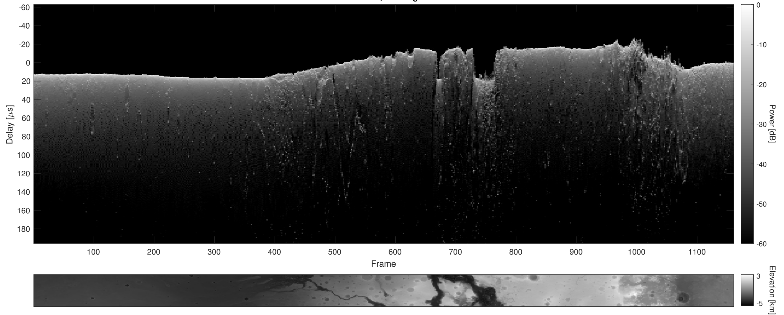
Orbit 15538, Cluttergram
