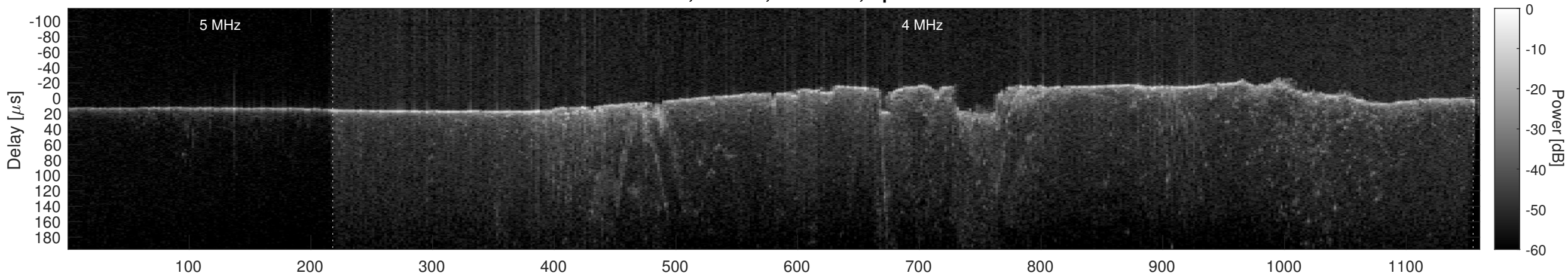
Orbit 15538, Cluttergram
