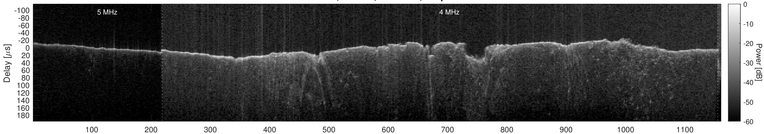
Orbit 15538, Window, Channel 1, Optimized
