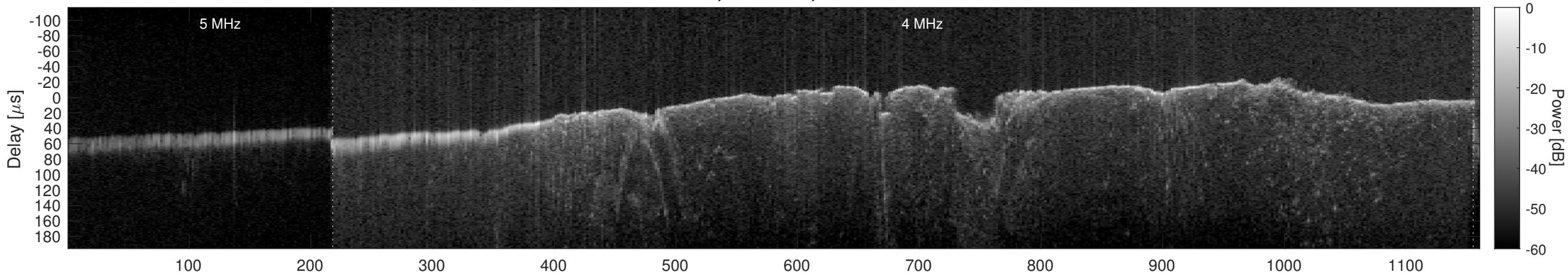
Orbit 15538, Window, Channel 1, Chapman
