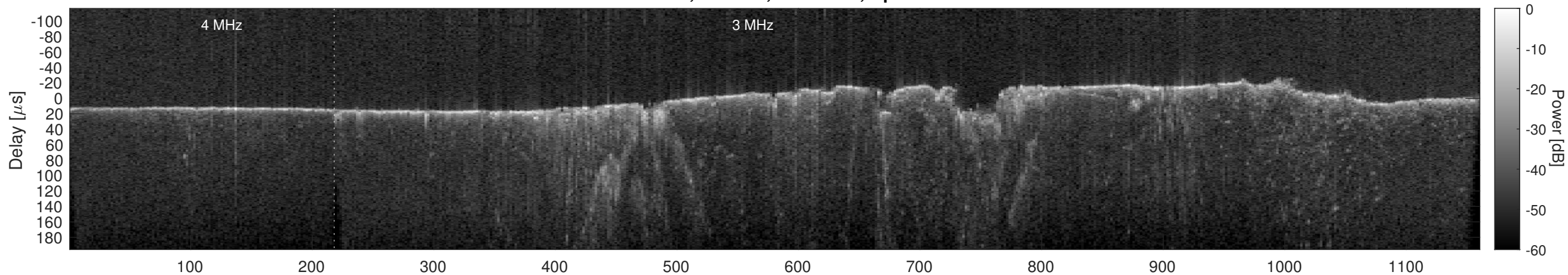
Orbit 15538, Cluttergram
