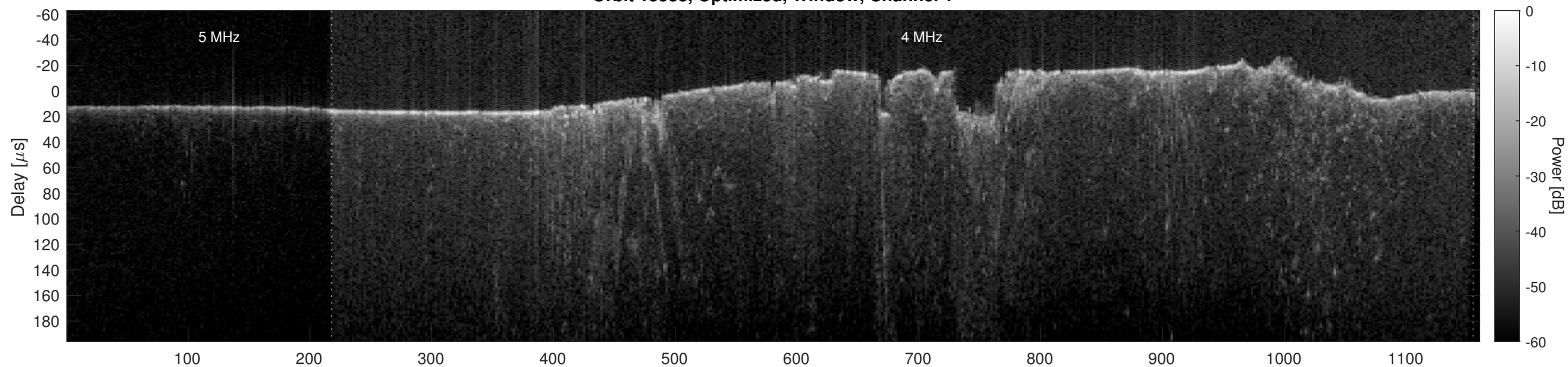
Orbit 15538, Optimized, Window, Channel 2
