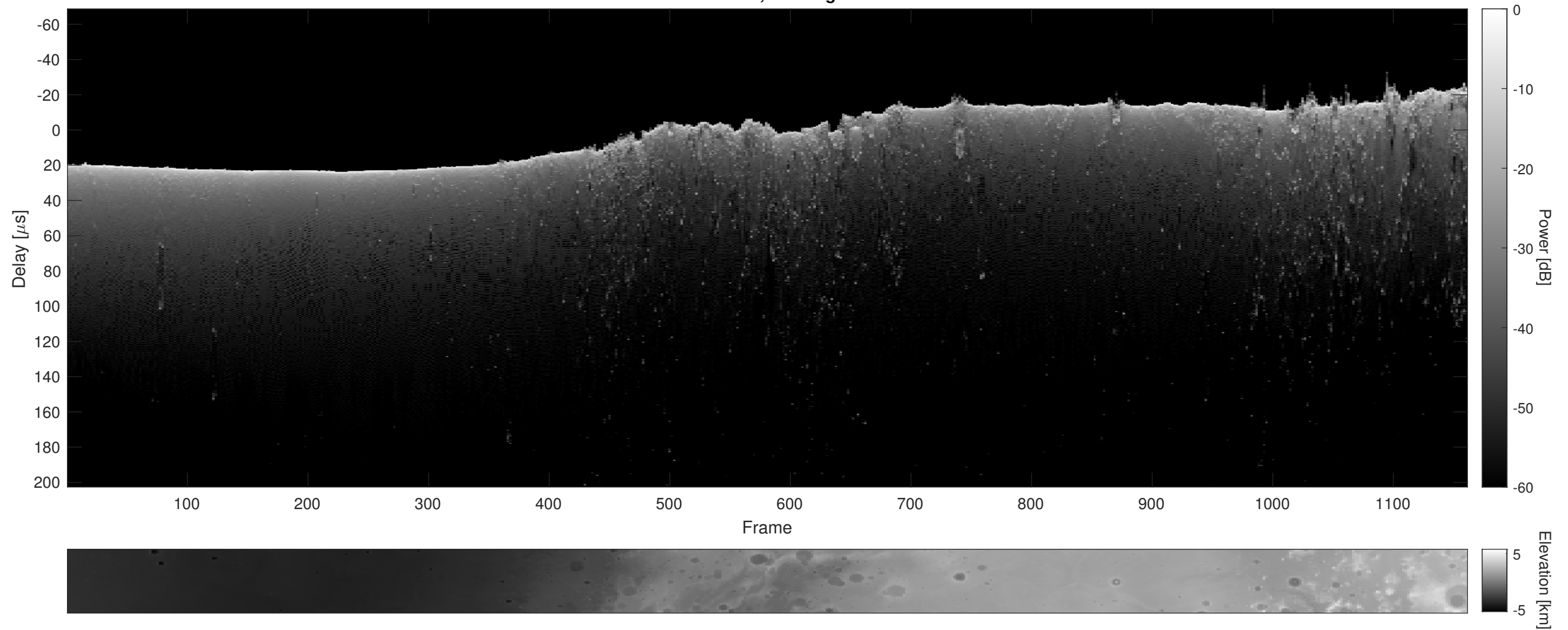
Orbit 15540, Cluttergram
