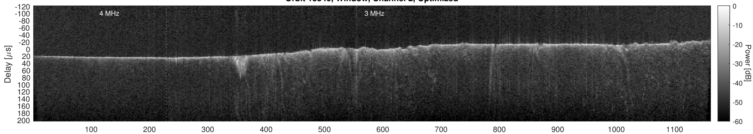
Orbit 15540, Cluttergram
