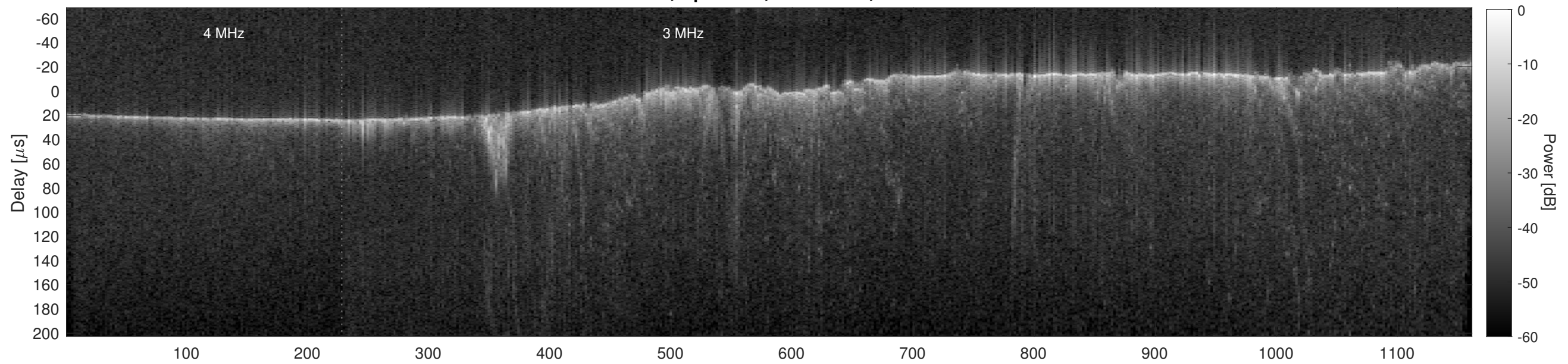
Orbit 15540, Cluttergram
