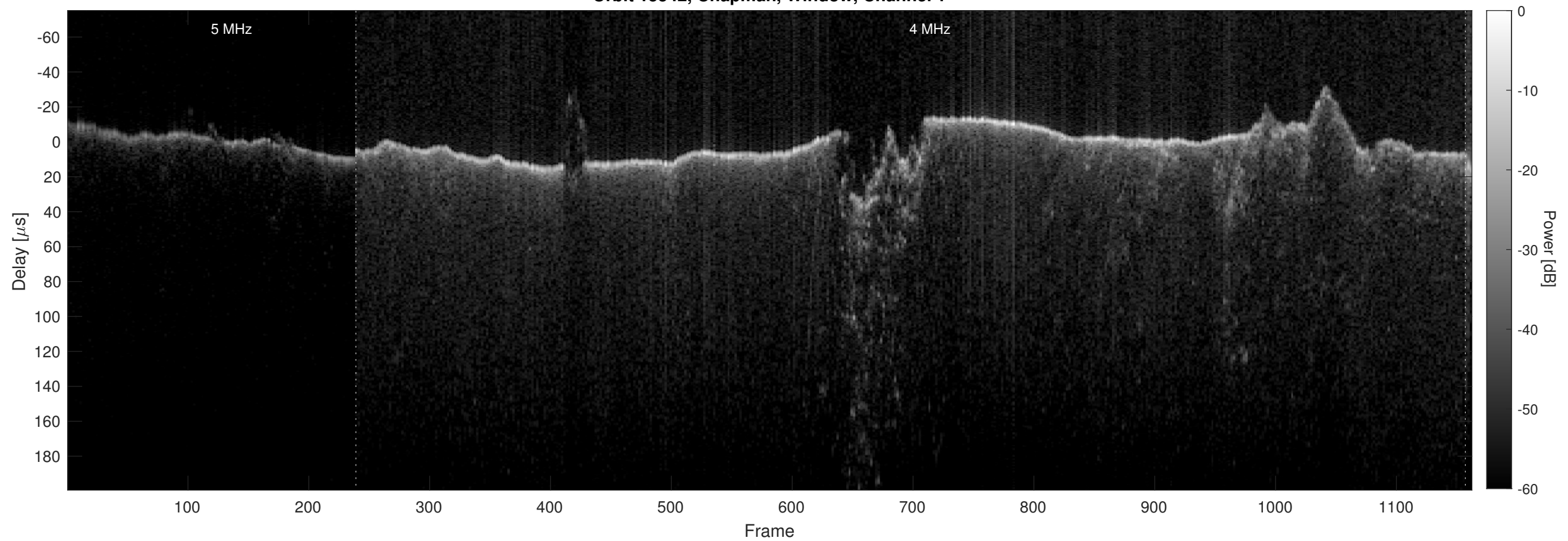
Orbit 15542, Chapman, Window, Channel 2
