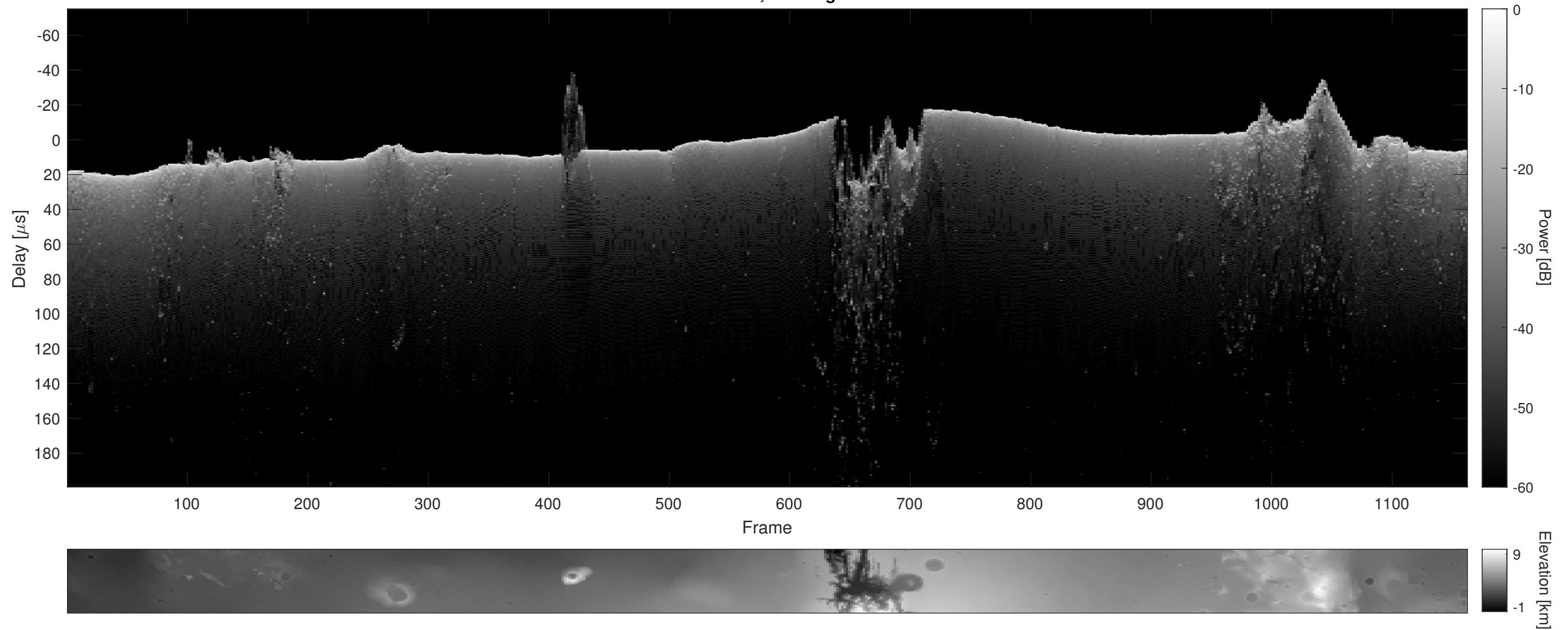
Orbit 15542, Cluttergram
