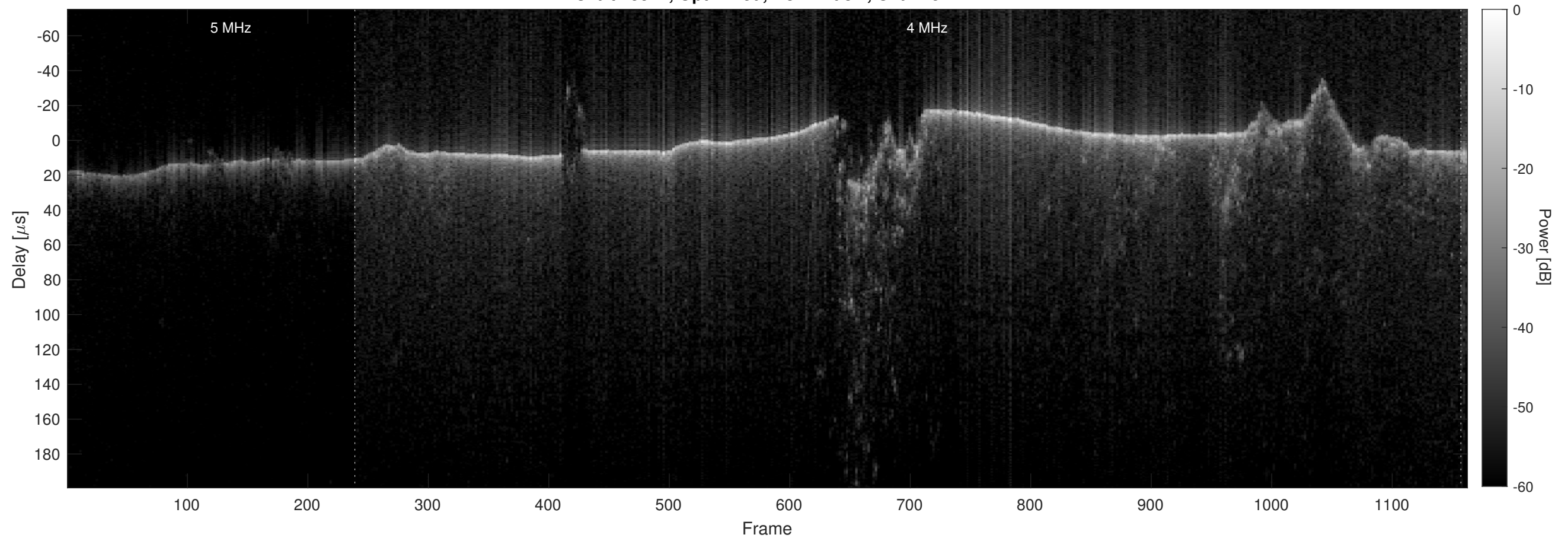
Orbit 15542, Optimized, No Window, Channel 2
