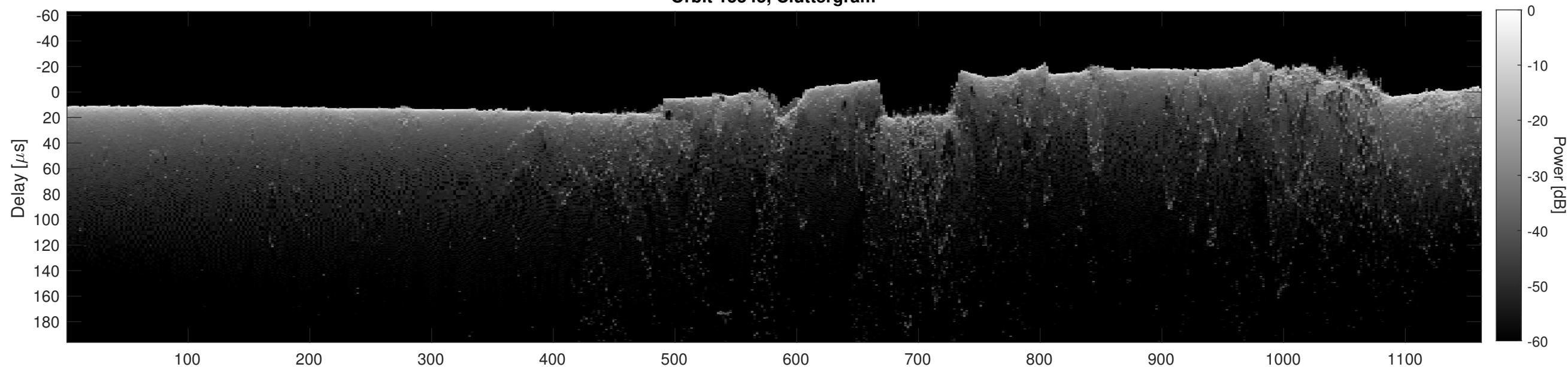
Orbit 15545, Cluttergram
