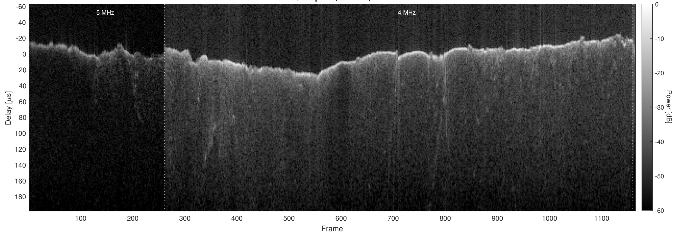
Orbit 15546, Chapman, Window, Channel 2
