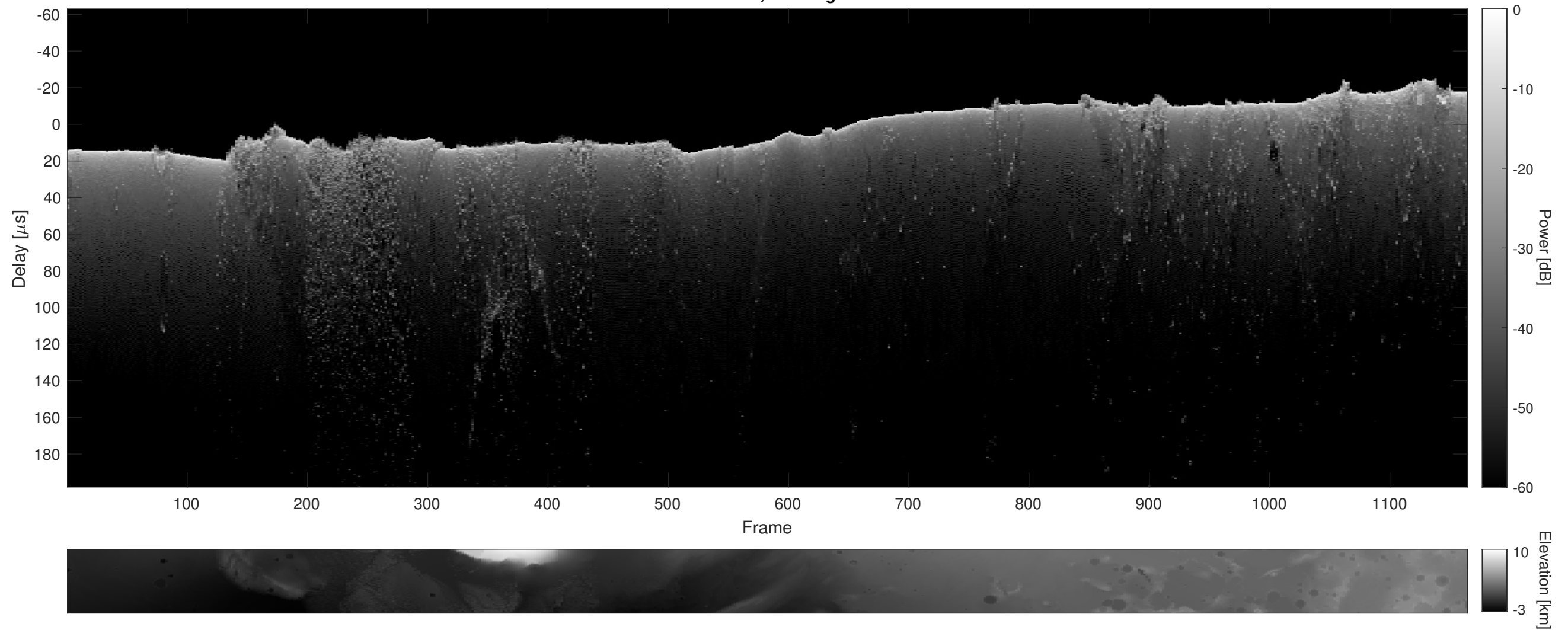
Orbit 15546, Cluttergram
