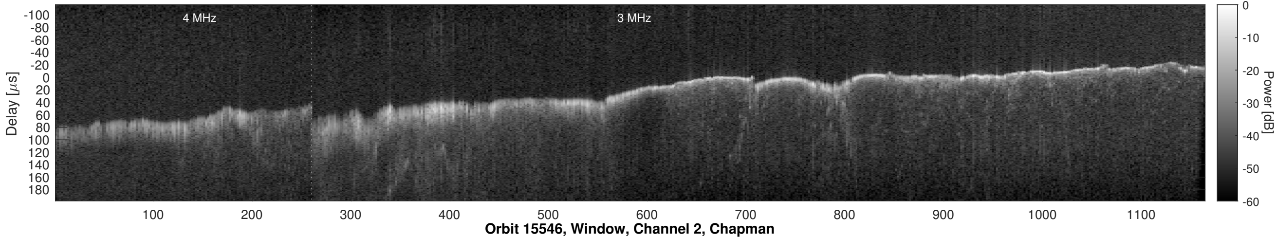
Orbit 15546, Window, Channel 2, Uncorrected
