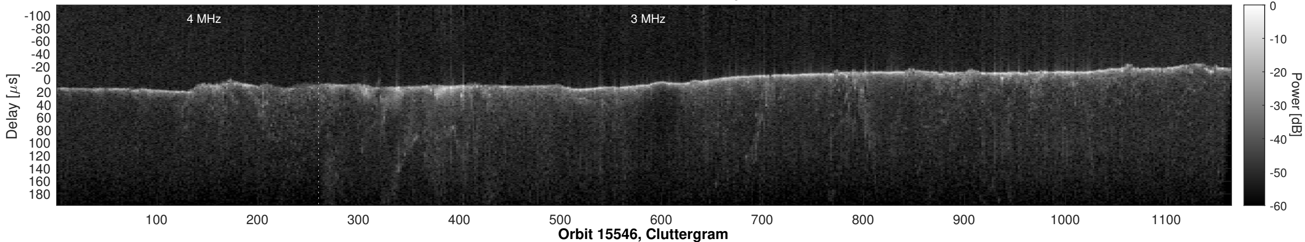
Orbit 15546, Window, Channel 2, Optimized
