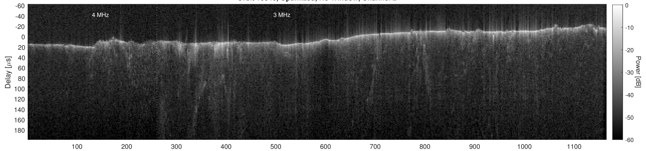
Orbit 15546, Cluttergram
