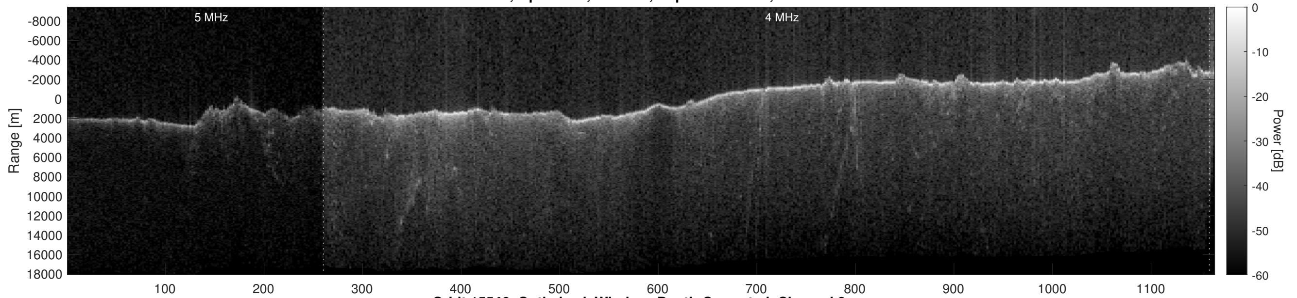
Orbit 15546, Optimized, Window, Depth-Corrected, Channel 2
