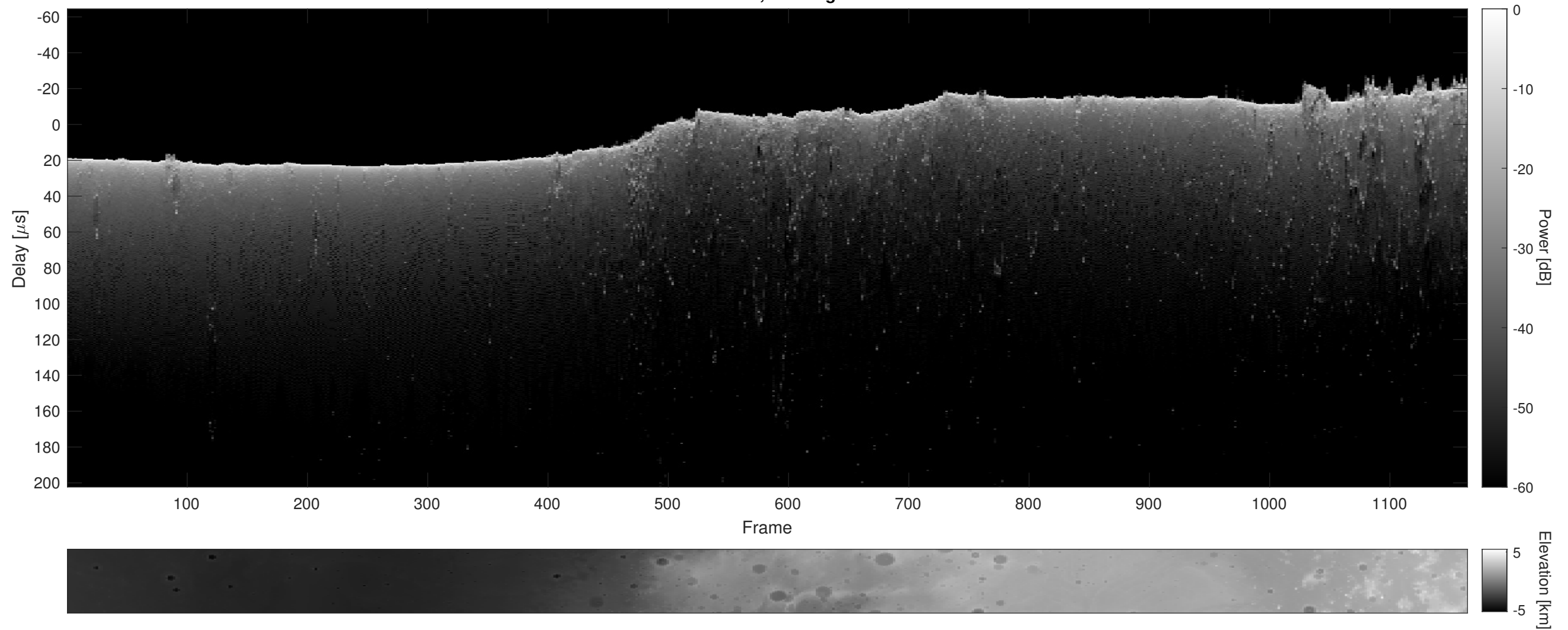
Orbit 15547, Cluttergram
