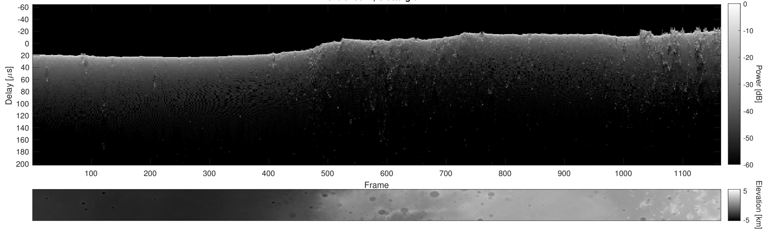
Orbit 15547, Cluttergram
