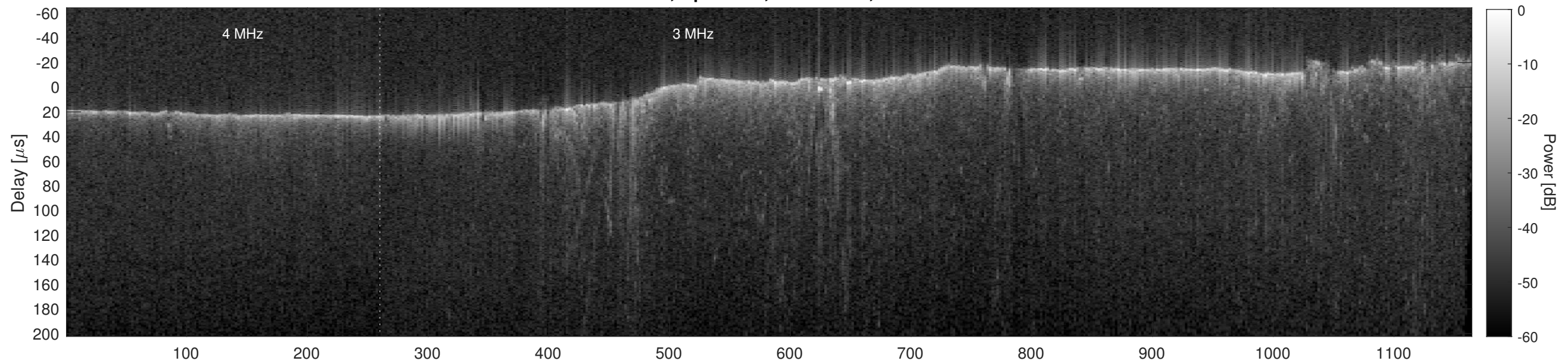
Orbit 15547, Cluttergram
