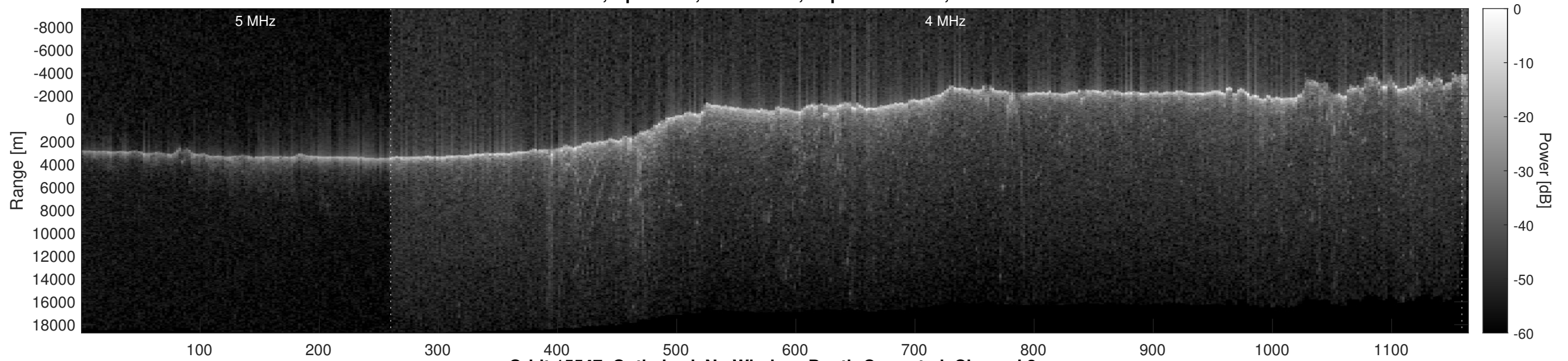
Orbit 15547, Optimized, No Window, Depth-Corrected, Channel 2
