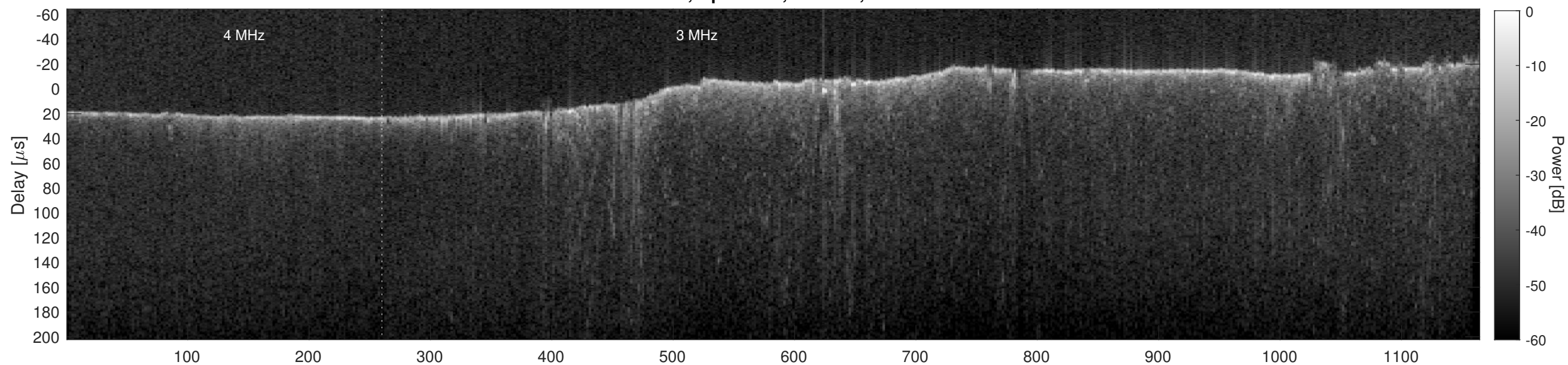
Orbit 15547, Cluttergram
