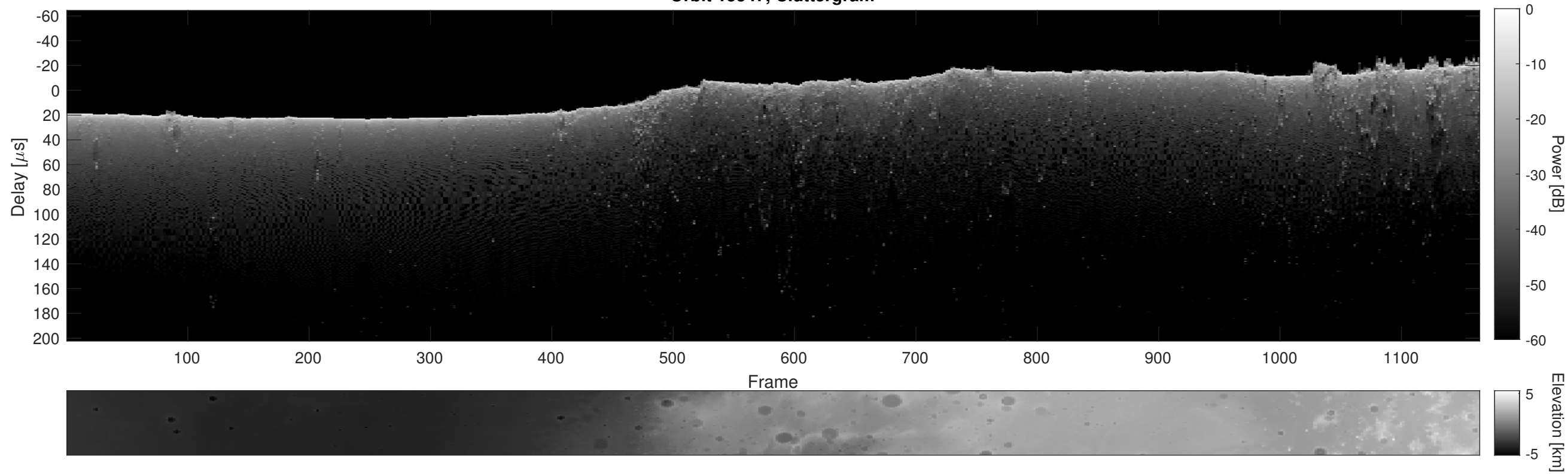
Orbit 15547, Cluttergram
