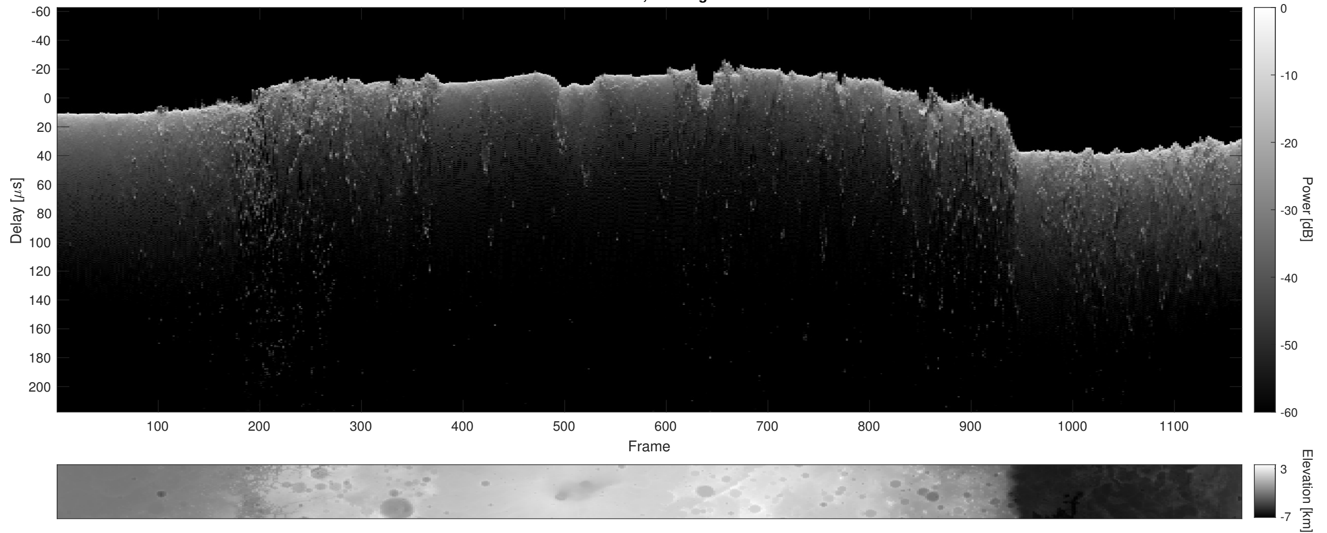
Orbit 15551, Cluttergram
