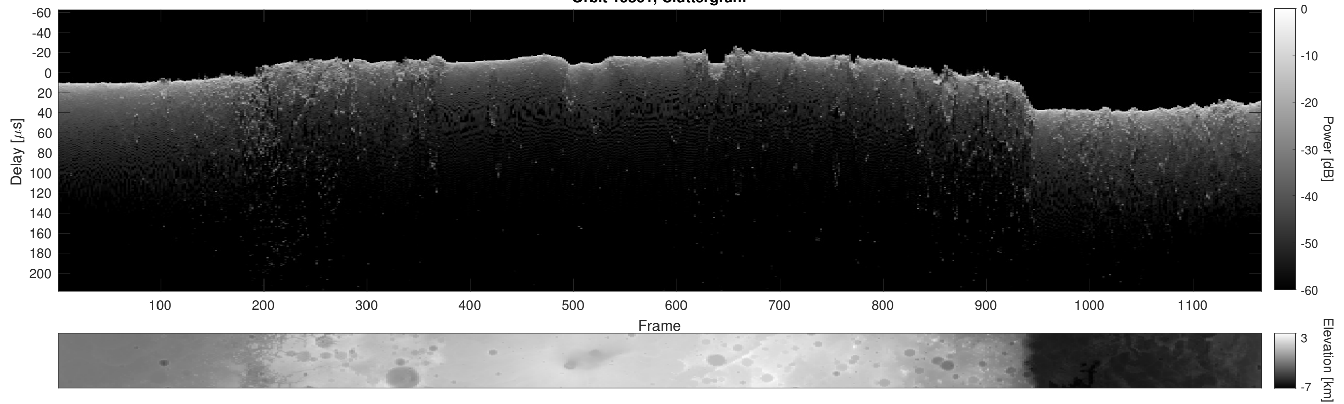
Orbit 15551, Cluttergram
