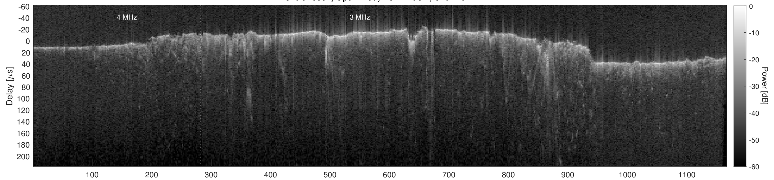
Orbit 15551, Cluttergram
