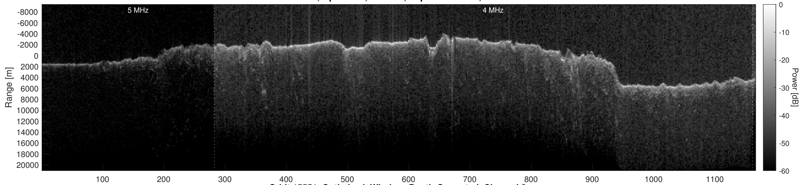
Orbit 15551, Optimized, Window, Depth-Corrected, Channel 2
