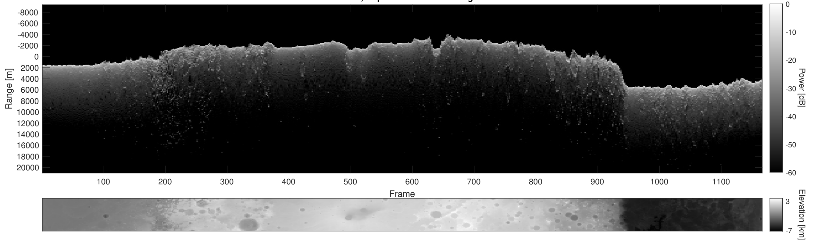
Orbit 15551, Depth-Corrected Cluttergram
