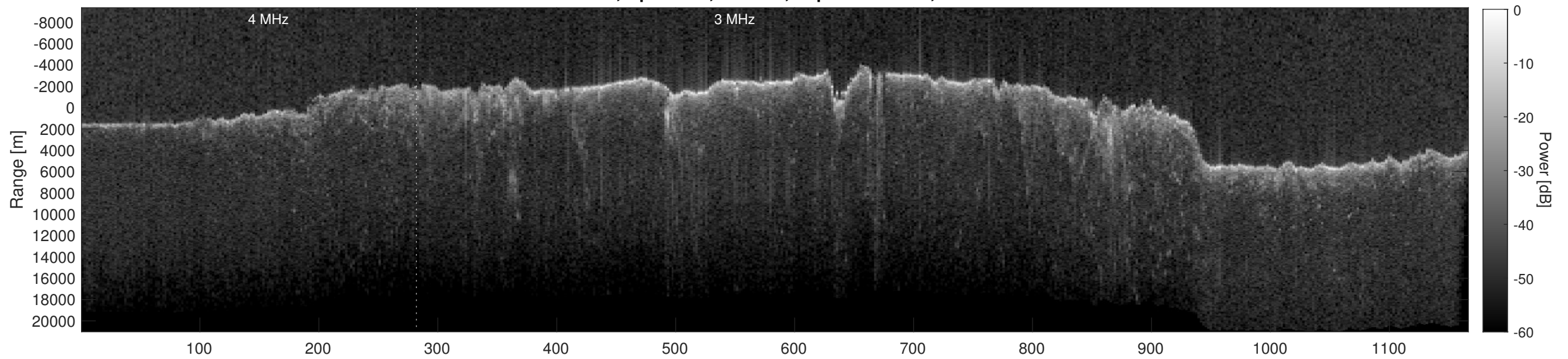
Orbit 15551, Depth-Corrected Cluttergram
