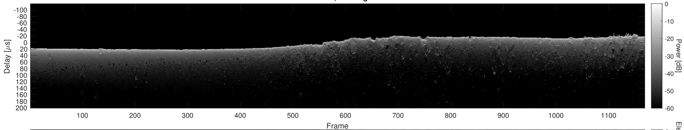
Orbit 15554, Cluttergram
