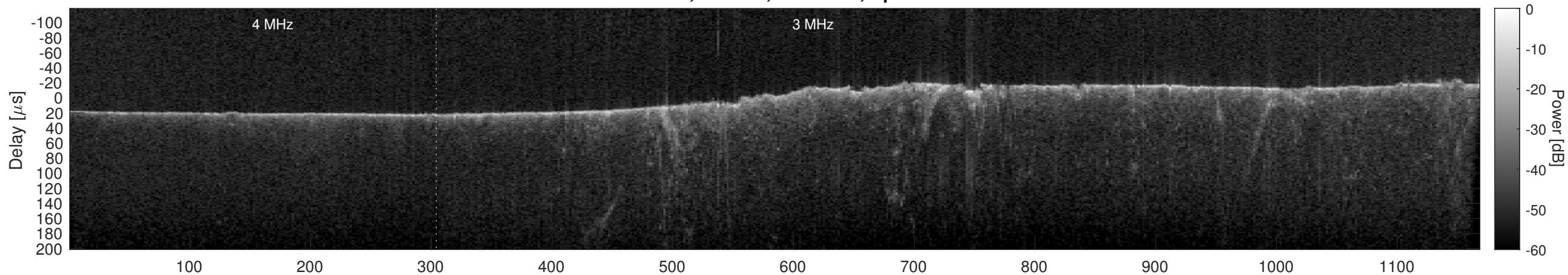
Orbit 15554, Cluttergram
