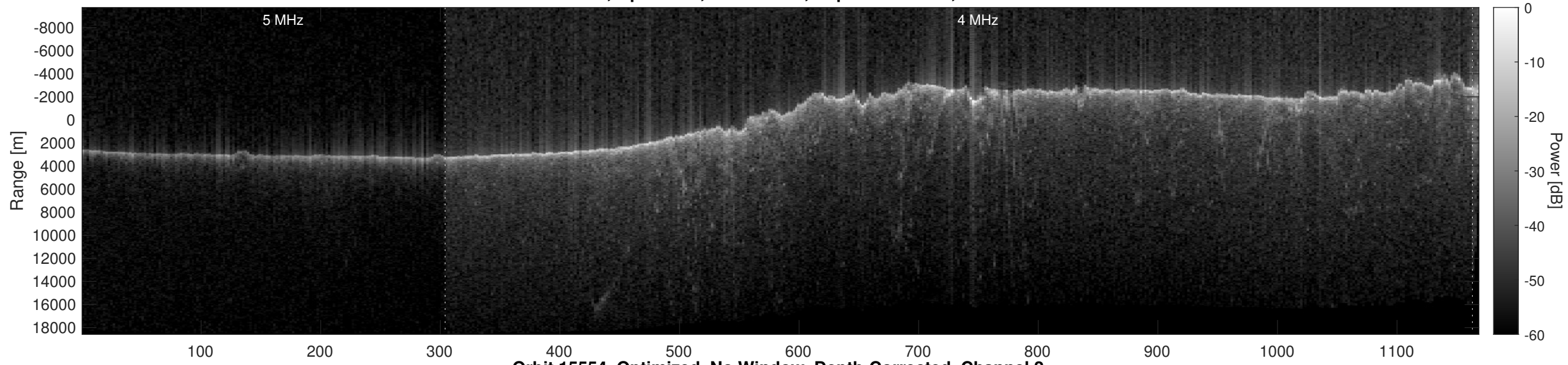
Orbit 15554, Optimized, No Window, Depth-Corrected, Channel 2
