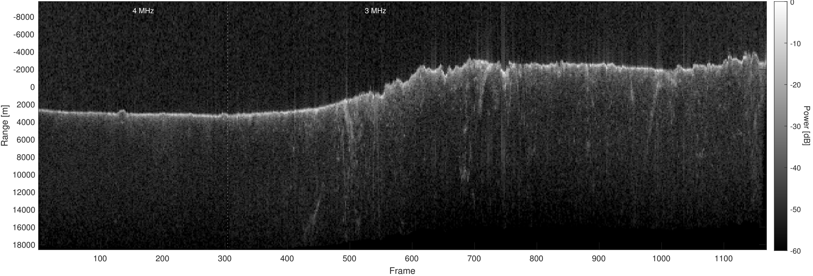
Orbit 15554, Optimized, Window, Depth-Corrected, Channel 2
