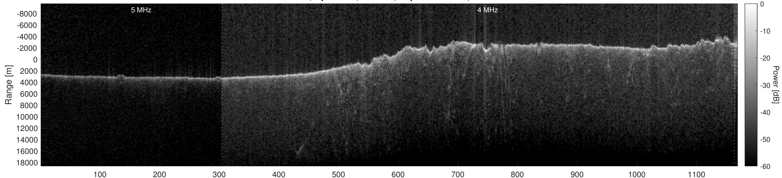
Orbit 15554, Optimized, Window, Depth-Corrected, Channel 2
