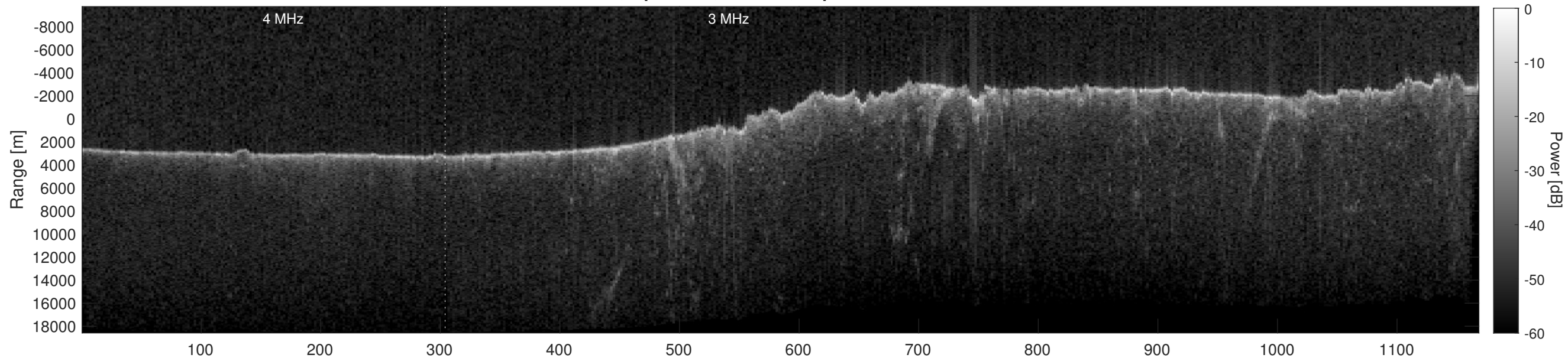
Orbit 15554, Depth-Corrected Cluttergram
